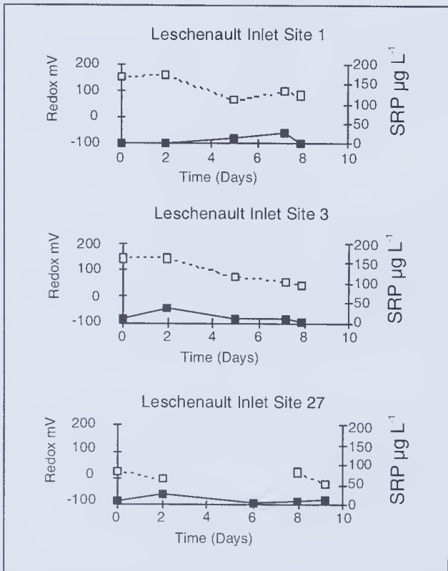
Figure 6. Phosphate (SRP) release and redox potential in intact cores collected in March 1990 from Leschenault Inlet. Site 1; Site 3; Site 27. - -□- - - Redox; —■— SRP.
